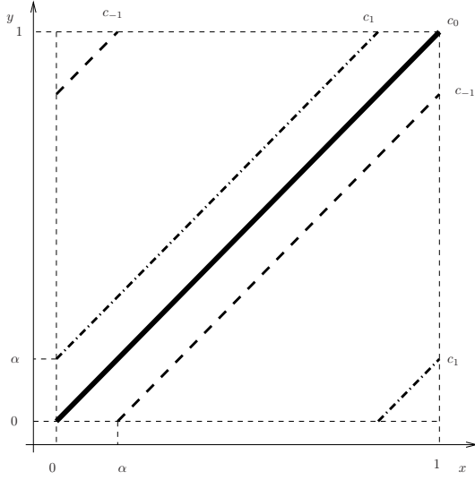
(a) When \alpha \notin \mathbb{Q} , the cycle decomposition of the plan \pi = (\text{Id}, \text{Id})_{\#} \mathcal{L}^1 gives only a consistent disintegration (Ex. 6.1).
