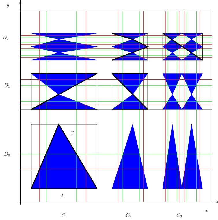
Figure 2: The set where A should be contained in order to have that A' is a subset of the standard order \leq on [0, 1] . The bold curves are the limbs of \Gamma , and two axial path are represented.
