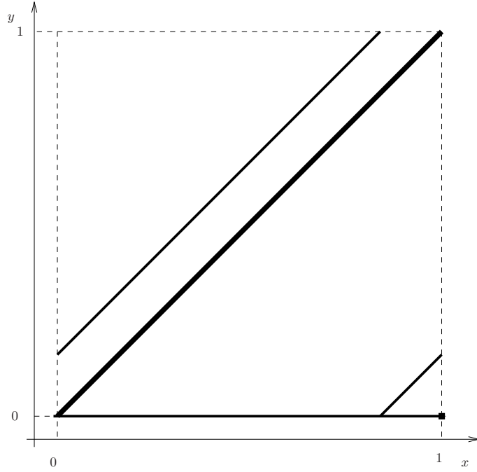
Figure 8: The cost function considered in Point (d) at Page 54
