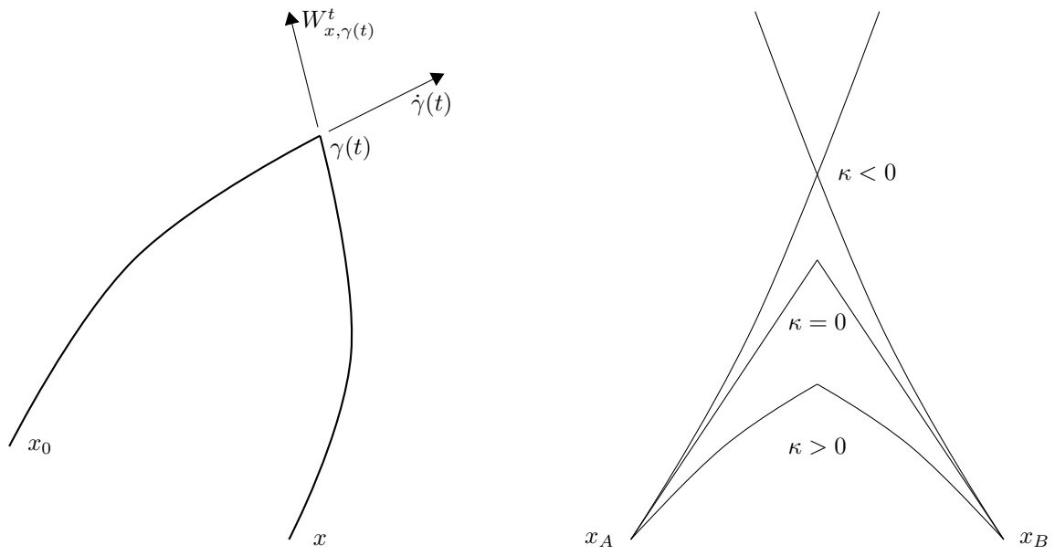
FIGURE 1. A geometrical interpretation for the function c_t .
