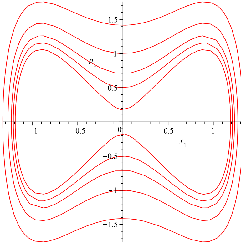
FIGURE 1. Phase portrait of the example (level sets of the Hamiltonian H )
