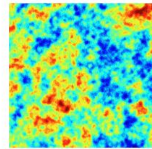
The Same 100 Square Degree Patch Cut From Each Full-Sky Map - WMAP - - Planck -
