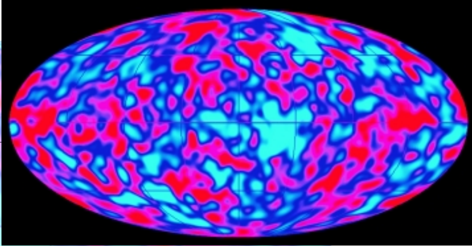
In 1992, NASA's COBE satellite confirmed for the first time that the temperature of the Cosmic Microwave Background (CMB) was not identical all over the sky. The COBE measurements indicated that over angular scales larger than 10^\circ , the CMB temperature varies by about one part in 100 000 from the average value of about 2.73 K. The image shows the map of the sky from which these conclusions were drawn.
