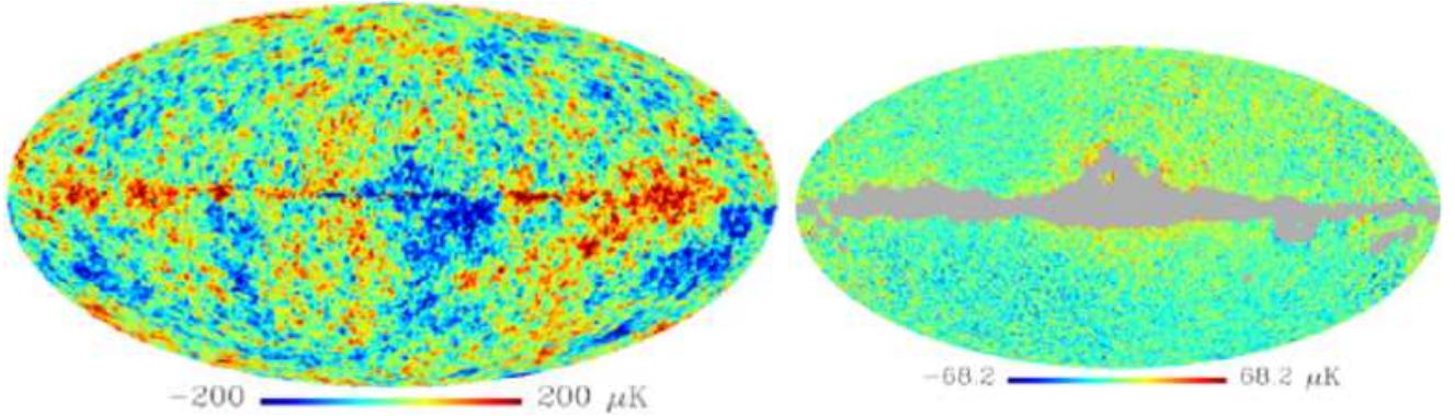
Figure 3. Left - CMB ICA map for full sky KKaQVW analysis. The residual along the Galactic plane is evident. Right - Difference between full sky and Kp2 ICA CMB maps: some residual Galactic signals is present near the edge of the sky mask and around some bright sources. High latitudes, large scale residual patterns are also present.
