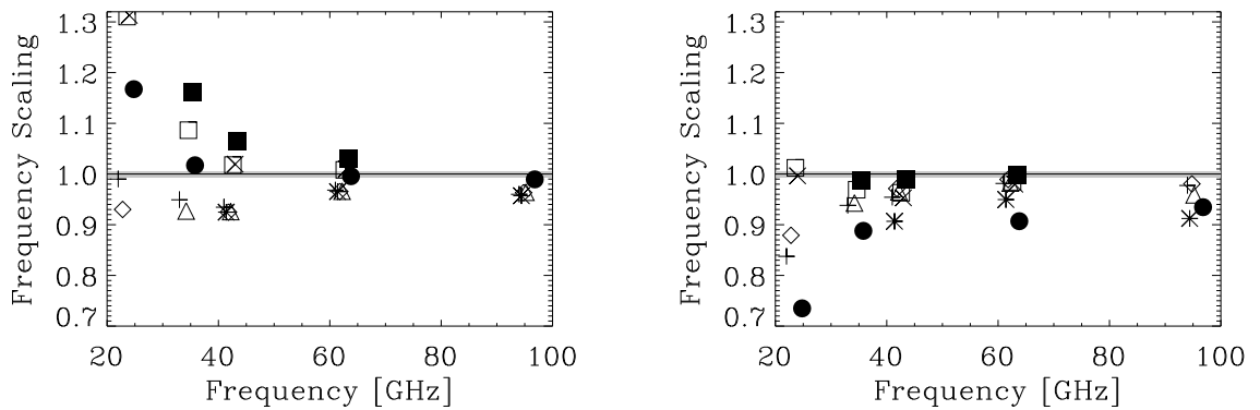
Figure 4. CMB frequency scaling for full-sky (left panel) and Kp2 analysis (right panel). Plus signs refer to KKaQVW combination, asterisks to QVW, rombs to KQVW, triangles to KaQVW, empty square to KKaQV, crosses to KQV, filled squares to KaQV and filled circles to KKaVW.
