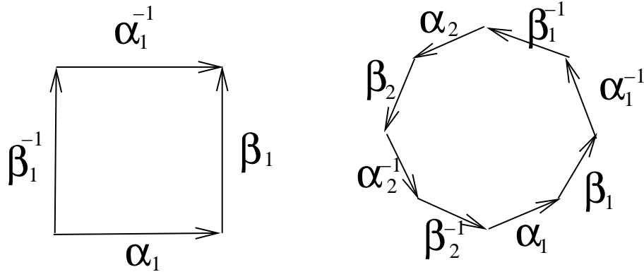
Figure 2.8: Poincaré polygon for surfaces of genus one and two.
