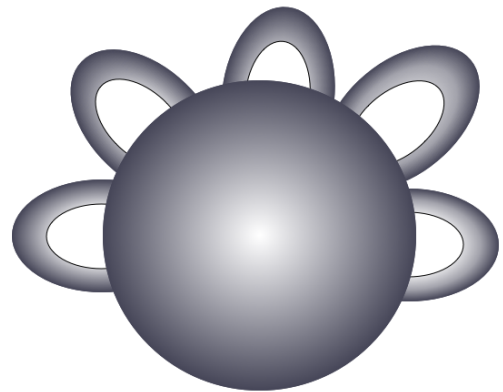
Figure 2.1: A sphere with five handles
