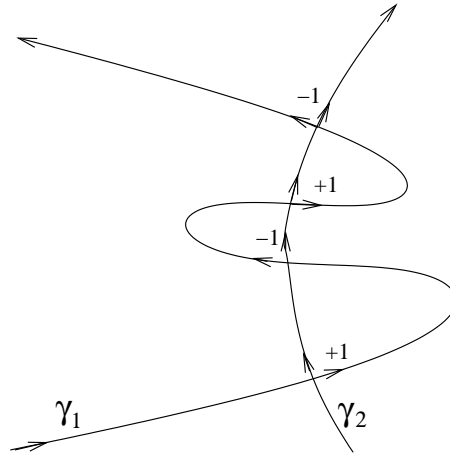
Figure 2.6: Intersection of \gamma_1 and \gamma_2 .
